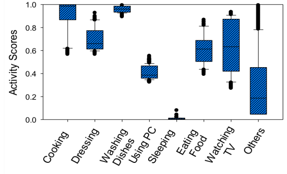
Figure 4. Activity scores according to home activities.
